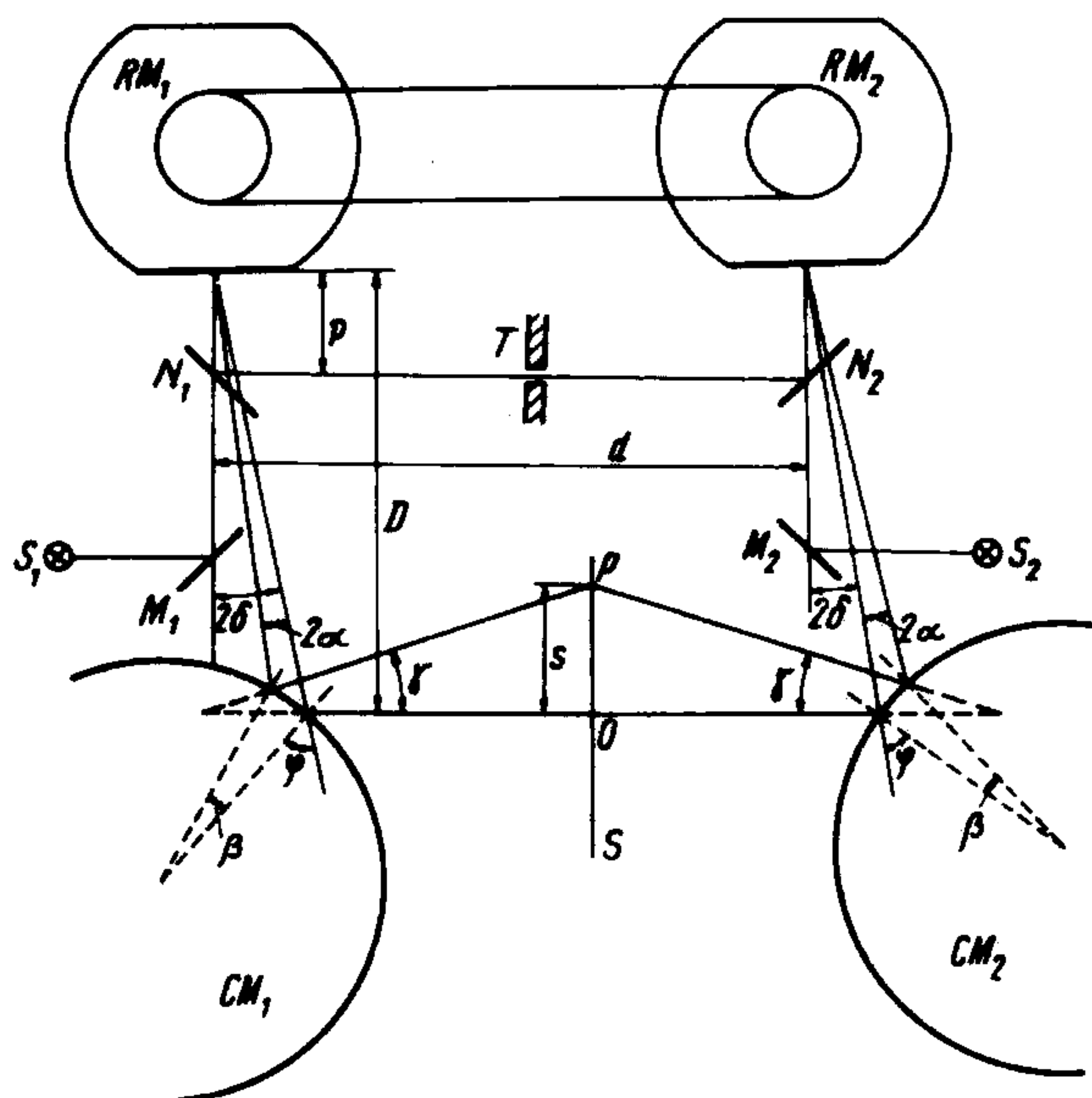
Fig. 1. The "coupled-mirrors" experiment.
